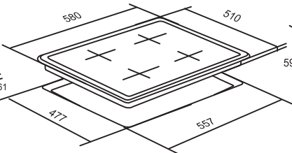
60cm Gas Hob Black Glass FAL-BGH-60
